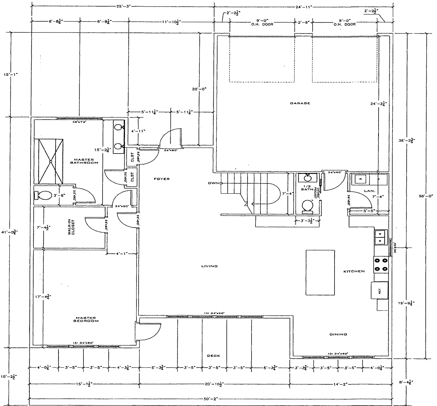
MAIN LEVEL FLOOR PLAN 1/4" = 1'-0"
